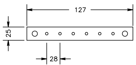
BUS BAR FOR ENTRANCE FACILITIES GROUND
