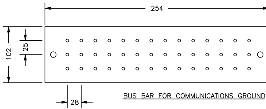
GROUND BUS BARS IN MAIN COMMUNICATIONS ROOM ( TMGB )
